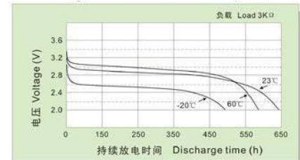
Discharge Characteristics on Temperature
