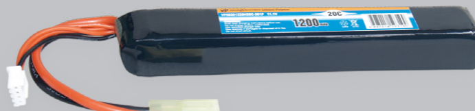
VP5820122SH20C-3S1P-11.1V 1200mAh with Tm1 Connector and 16# Silicone Wires Dimension: 17mm*20mm*127mm Weight: 102g Burst Discharge Current: 30C
